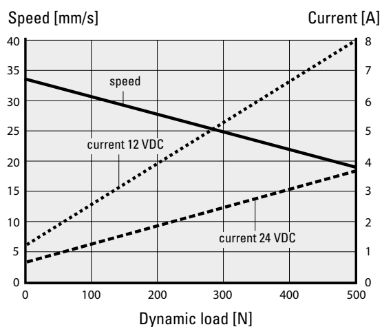
Worm Screw Models (MX • • W)
